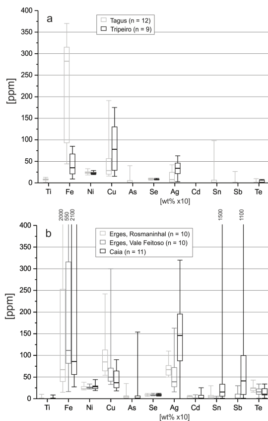
Figure 3. Variation of minor and trace elements in gold from (a) the Tagus palaeo-placer and Tripeiro placer, as well as (b) the Erges and Caia placers. Concentrations are in ppm, except for Ag and Au. n = number of data sets acquired.
