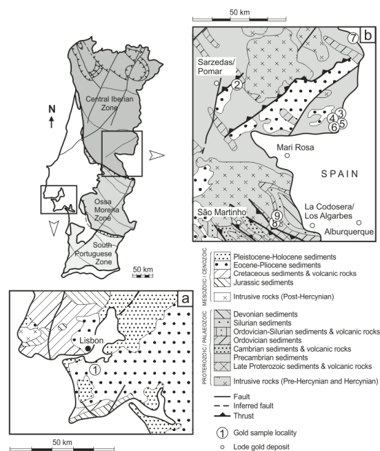
Figure 1. Locality maps of the study area, modified after the Carta Geológica de Portugal Scale 1:500.000 (1992). (a) Simplified geological map of the Tagus estuary containing the Tagus palaeo-placer (1). (b) Simplified geological map of the southern CIZ and BCSZ in the Castelo Branco region containing the Tripeiro (2), Erges, Rosmaninhal (3-6), Erges, Vale Feitoso (7), and Caia (8-9) gold placers.
