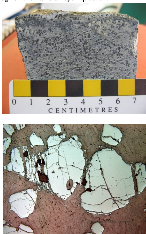
Figure 2. Disseminated chromite in handspecimen sample of disunite collected in one of the many mine dumps (above) and photomicrograph of the chromite grains in thin-section (below; both samples are from the Valongo area).
