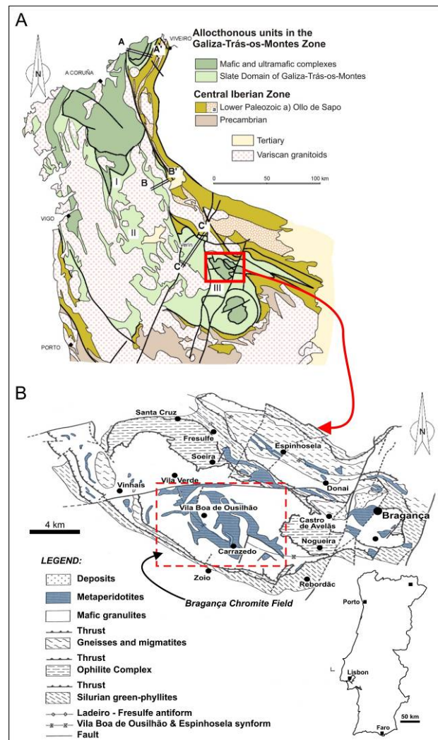
Figure 1. A- Allochthonous units of the Galiza - Trás-os-Montes Zone (after Arenas et al. 2004) and B - Geological map for the Bragança Massif showing the divisions between the main tectonic units (After Prichard et al. 1991).
