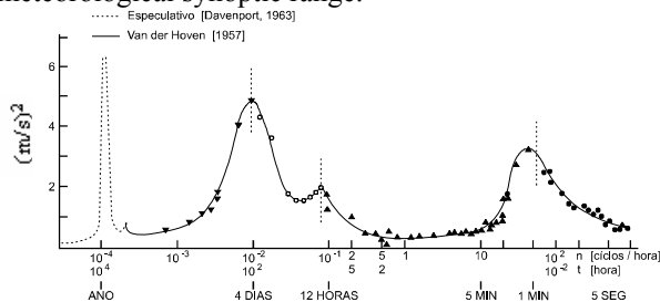
Fig. 2. The van der Hoven wind spectrum was measured by the author in the fifties at the Broohaven National Laboratory and is still used as reference for wind engineering worldwide. It is also used in several national codes for the wind actions on structures. [8].
