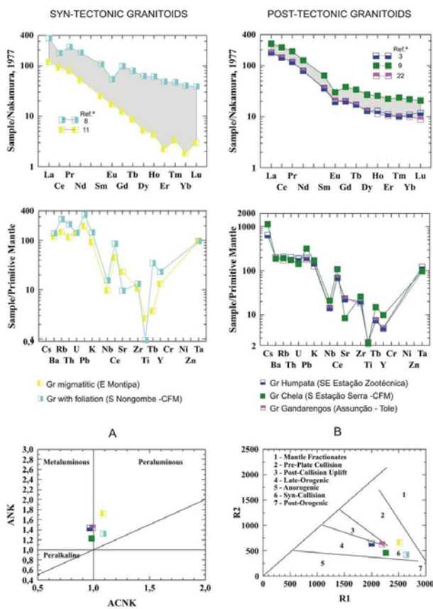
Fig. 4. Chondrite-normalized REE patterns (Nakamura, 1977) of syn and post-tectonic Eburnian granitoids from the Lubango-Bibala region; multielementary diagrams sample / primitive mantle of syn and post-tectonic Eburnian granitoids from the Lubango-Bibala; A) A/CNK - A/NK , (Maniar & Picoli, 1989); B) R1=4Si-11(Na+K)-2(Fe+Ti) , R2=6Ca+2Mg+Al , (Batchelor & Bowden, 1985).
