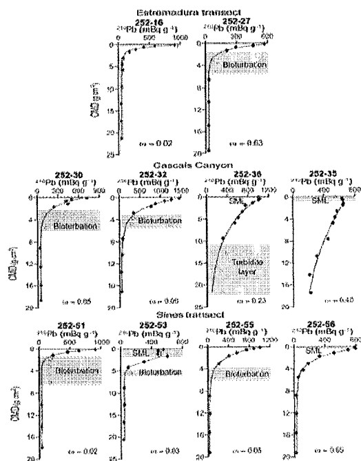
Fig. 2. Total 210 Pb activity vs. cumulative mass depth (CMD) and best-fit curve for determination of MAR. Open circles were not considered to the determination of MAR. MAR are given in g\text{ cm}^{-2}\text{ y}^{-1} .
