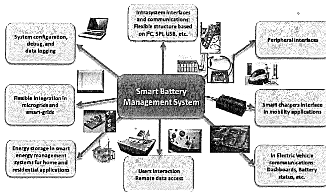
Figure 2. Smart Battery Management Systems communications interactions.
