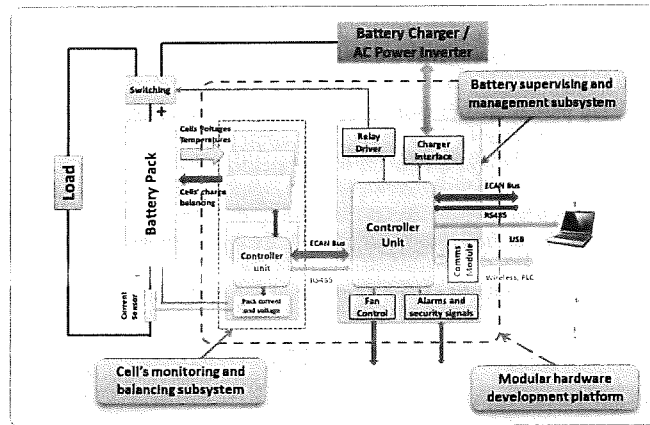
Figure 4. Global framework hardware architecture.
