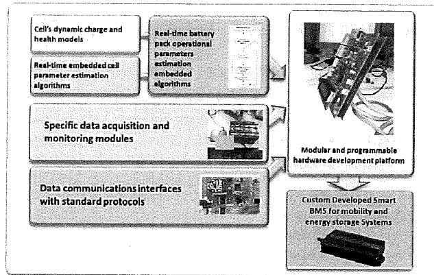
Figure 3. Global framework development environment
