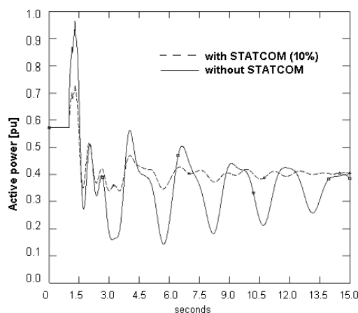
Fig. 10 – Active power flow in the interconnections, following a short circuit in a relevant transmission bus – with and without STATCOM (Franco Marques and Peças Lopes, 2006).
