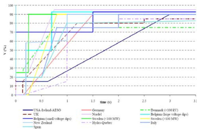
Fig. 2. LVRTF requirements for various grid codes (Tsiliet al , 2009)
