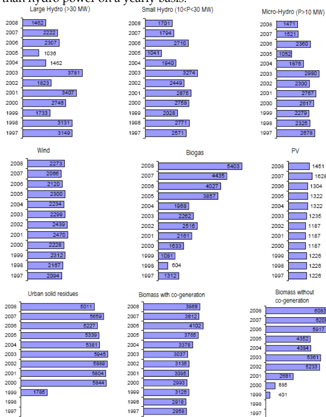
Fig.7. Comparison of annual equivalent production hours of different renewable sources (source: DGE, 2009)
