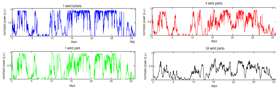
Fig. 1. Wind Power variability and aggregation smoothing effect
