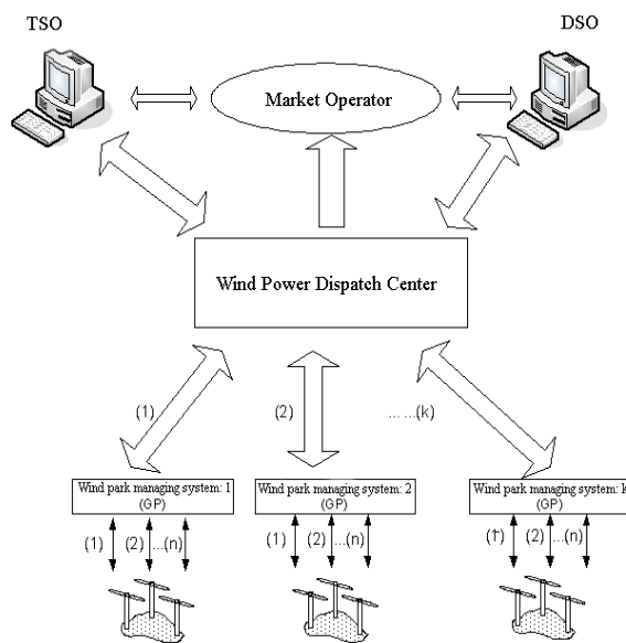
Fig. 5 - A possible architecture for the management of the power system with wind aggregation agents (Estanqueiro et al, 2007).
