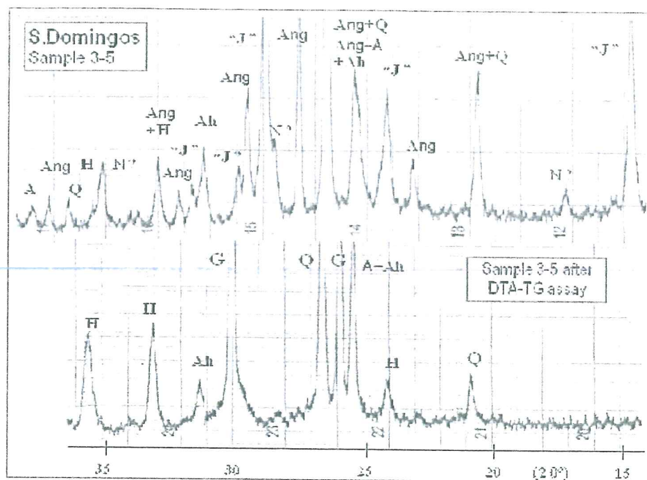
Fig. V.4 - XRD pattern of sample 3-5: above, as collected; below, after the thermal assay. Ang - anglesite ( \text{PbSO}_4 ); "J" - jarosite ( (\text{K}_{1-2}\text{Pb}_x)\text{Fe}_3(\text{SO}_4)_2(\text{OH})_6 ); Q - quartz ( \alpha\text{-SiO}_2 ); Ah - anhydrite ( \text{CaSO}_4 ); H - hematite ( \alpha\text{-Fe}_2\text{O}_3 ); A - anatase ( \text{TiO}_2 ); G - galena ( \text{PbS} ); N? Non identified minor phase.
