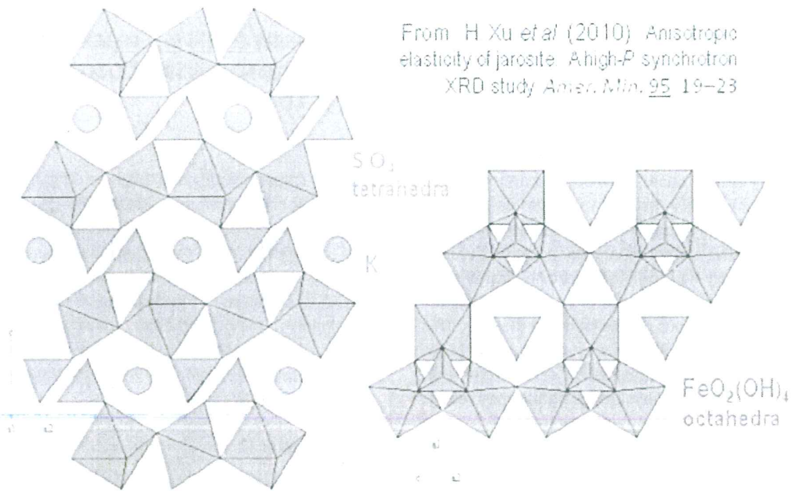
Fig. V.1 - Crystal structure of Jarosite [Modified from H. Xu et al. (2010) Anisotropic elasticity of jarosite: a high- P synchrotron XRD study. Amer. Min. 95, 19–23]
