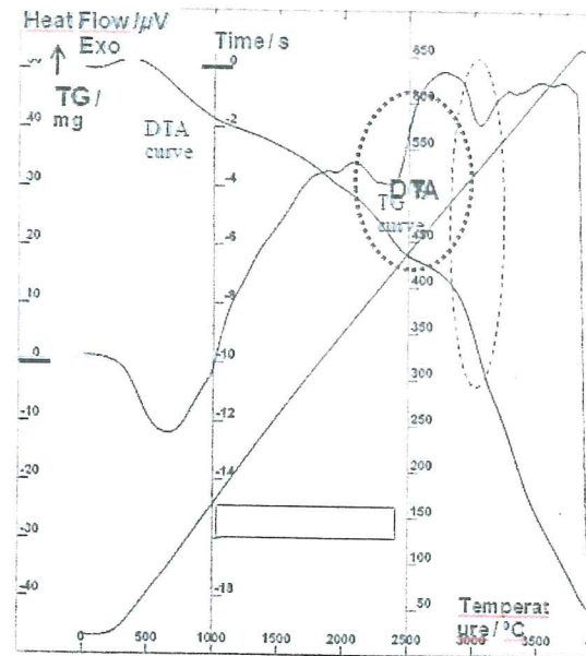
Fig. V.3 - Thermal analysis output. The regions corresponding to the decomposition of jarosite with liberation of water just above 450°C and to the release of SO_2 at higher temperature are assigned in DTA plus TG curves.
