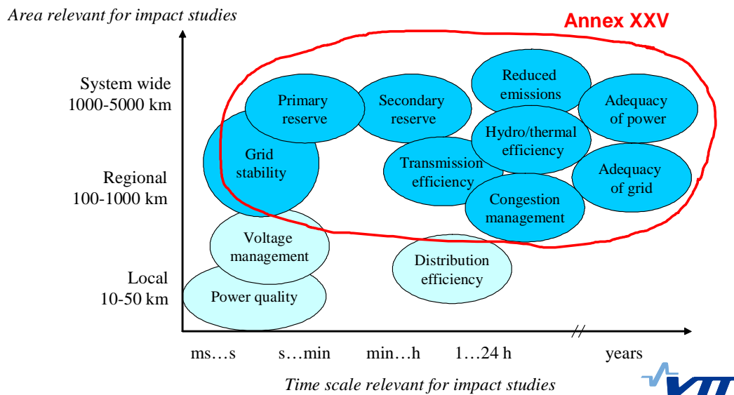
Figure 1. Impacts of wind power on power systems, divided in different time scales and width of area relevant for the studies. In this international collaboration (IEA WIND Annex 25), local issues of grid connection like power quality are not addressed but the more system related issues.
