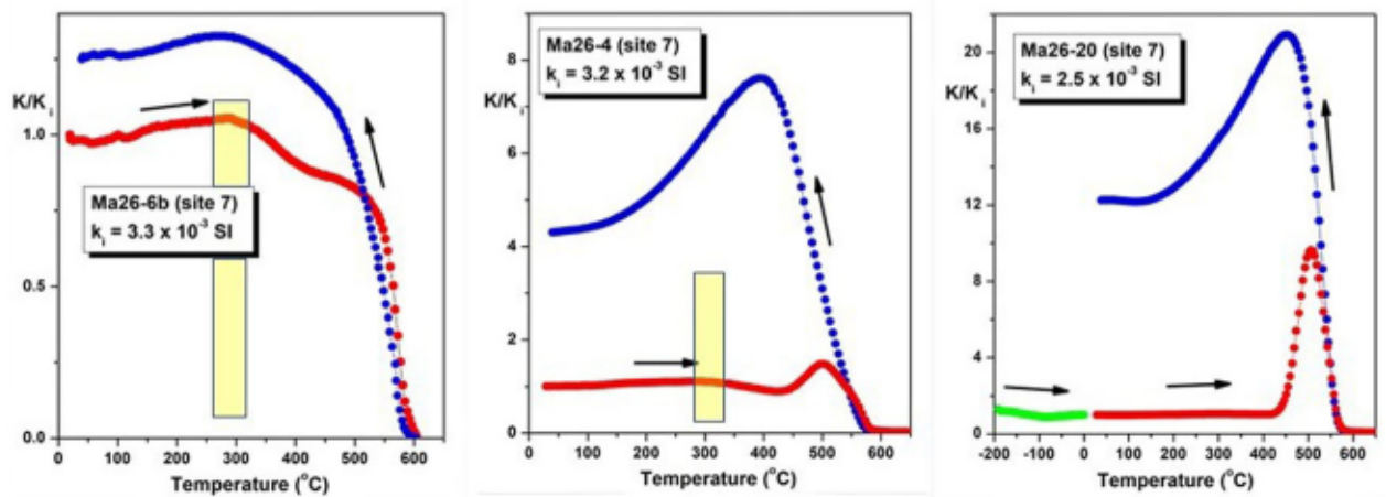
Figure 10. Representative k(T) curves of the of thermomagnetic behaviour of carbonatite samples from dike 26.
