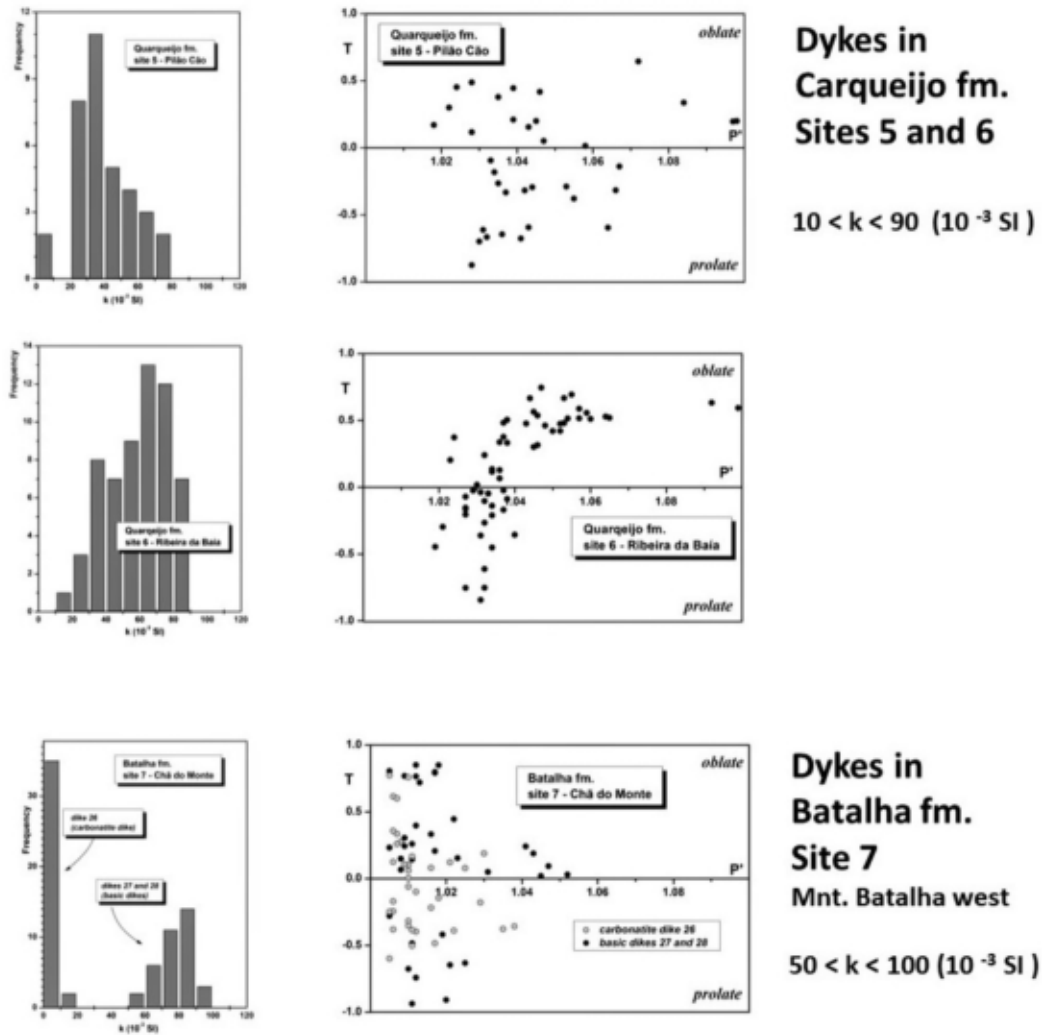
Figure 5b. Magnetic susceptibility distribution on dykes (left) and diagram of anisotropy degree P_j versus shape parameter T (right), sites 5, 6 and 7.
