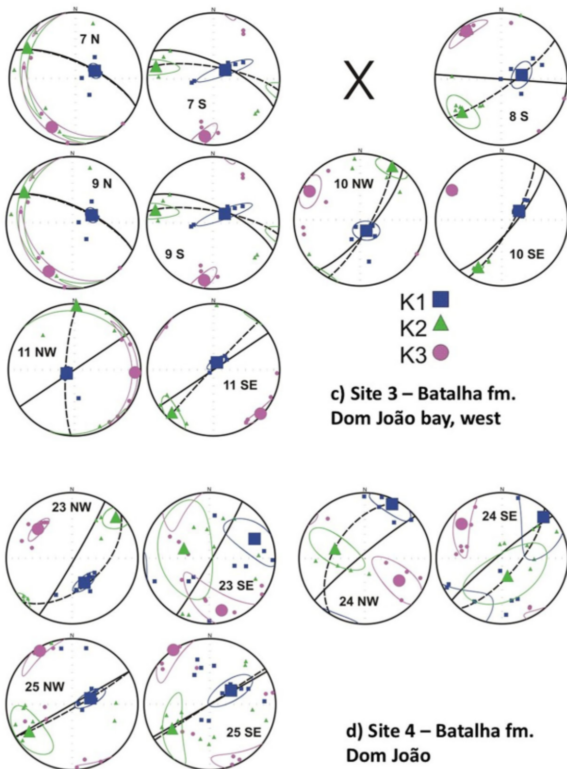
Figure 6b. Sites 3 and 4 (see previous caption).
