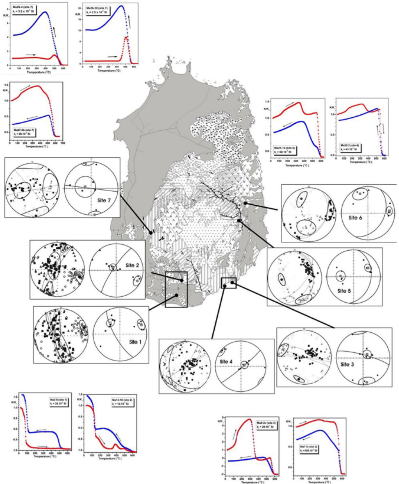
Figure 16. Synthesis of AMS results for all studied dikes in Maio. For each site we show two stereoplots. The left stereoplots shows the AMS results ( k_1 , k_2 and k_3 ) in the real (field) orientation of the grouped dikes with similar attitudes (differences in direction and dip < 20^\circ ). The right stereoplots represents the result of the rotation of the different dikes and mean magnetic directions (only k_1 and k_3 ) for a common referential. This referential is represented in the stereoplots by a 'synthetic' dike with the average orientation of the sampled dikes in that site. The corresponding magnetic axes of each dike were also rotated accordingly.
