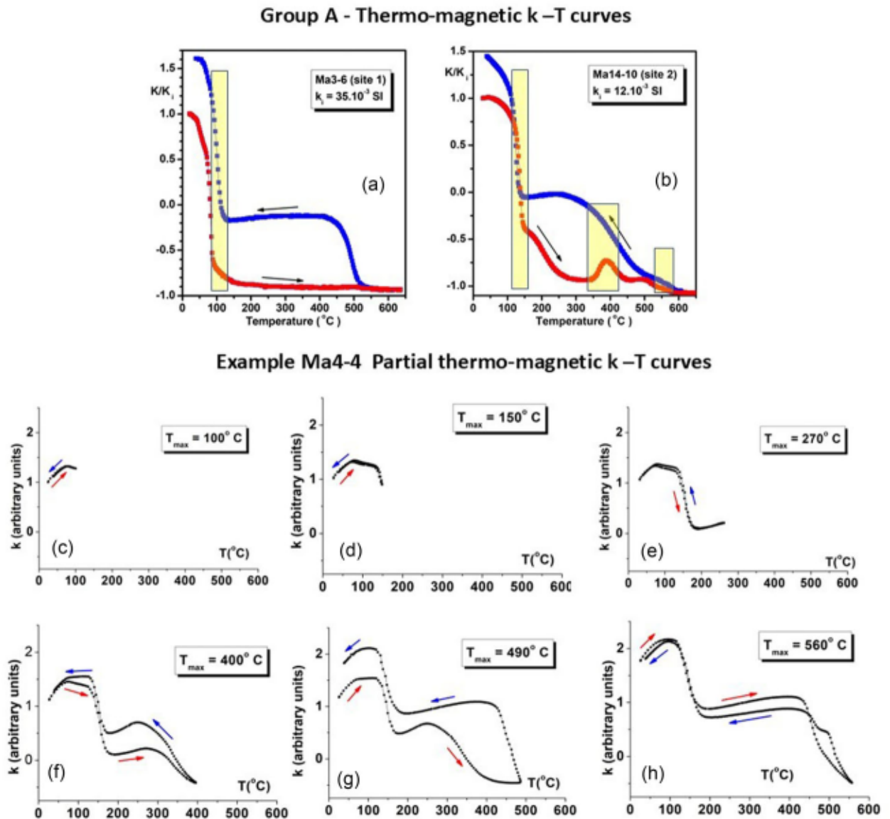
Figure 7. Representative k(T) curves of the thermomagnetic behaviour of group A samples (7a and 7b) and a representative partial thermomagnetic k(T) cycle for Ma4.4.
