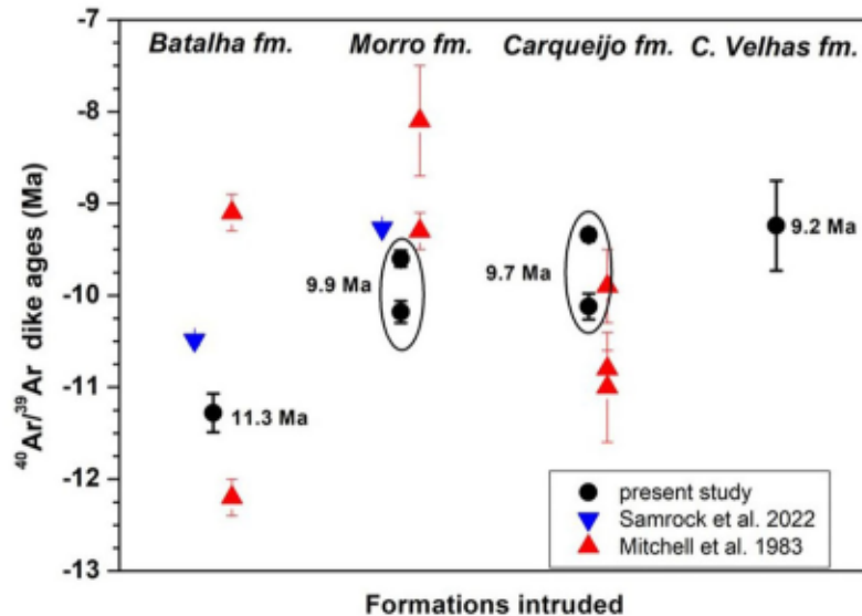
Figure 13. Compilation of K–Ar and ^{40}\text{Ar}/^{39}\text{Ar} ages of dikes from Maio Island from Mitchell et al. 1983 and Samrock et al. 2022, and the new ^{40}\text{Ar} – ^{39}\text{Ar} ages obtained in this study. The 2\sigma errors are indicated by error bars. Data points encircled represented different ages from different dikes intruding the same formation. The obtained ages are indicated.
