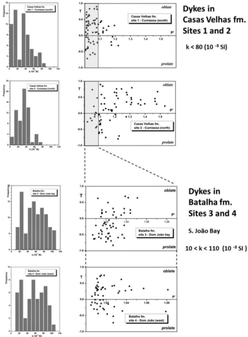
Figure 5a. Magnetic susceptibility distribution on dikes (left) and diagram of anisotropy degree P_j versus shape parameter T (right), sites 1, 2, 3, 4.
