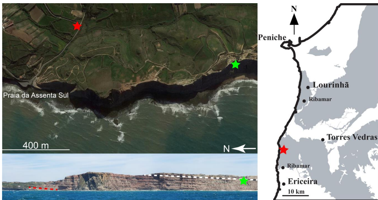
Figure 2. Regional simplified geological map (right), with location of Dracopelta zbyszewskii (red star). Gray coloured areas on the right represent Late Jurassic units. Satellite (top left) and coastal profile (bottom left) photographs of the Praia da Assenta Sul area. Green star indicates the site of the new ankylosaurian specimen FCT-UNL 702; white dashed line on bottom left represents approximate J-K boundary according to Mateus et al. (2017); red dashed line marks the coastal equivalent unit to the type locality. Satellite image modified from Google Earth® and panoramic photo of the coast by André Carvalho.
