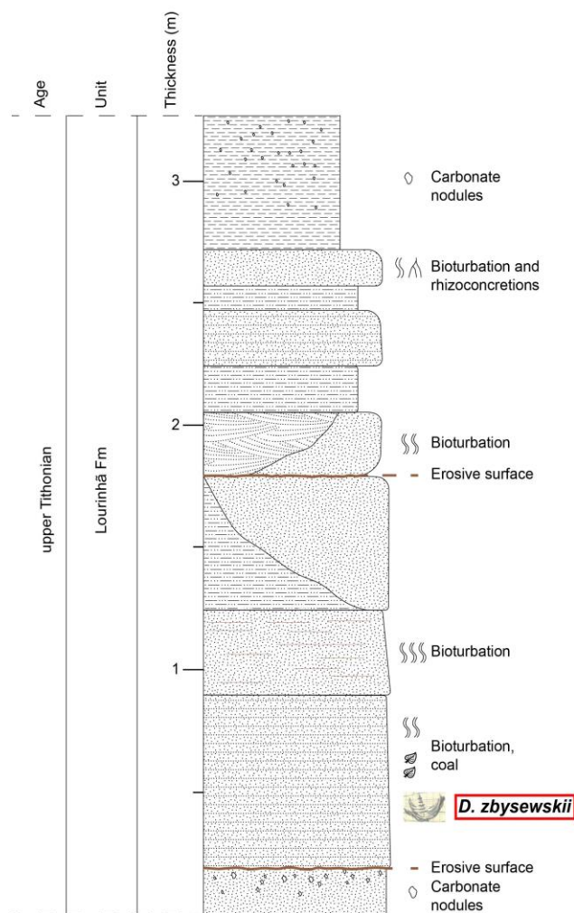
Figure 4. Type locality of Dracopelta zbysewskii (above) and local stratigraphic log showing the placement of the holotype in the section (below).
