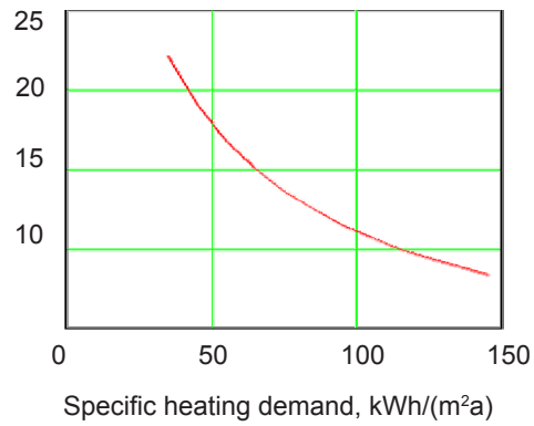
Figure 4. Line density as a function of energy retrofit standard (left) and the resulting specific costs of heat distribution (€/MWh, right). Line density is defined as the amount of thermal energy transported through the neighbourhood distribution grid in MWh/(m a).
