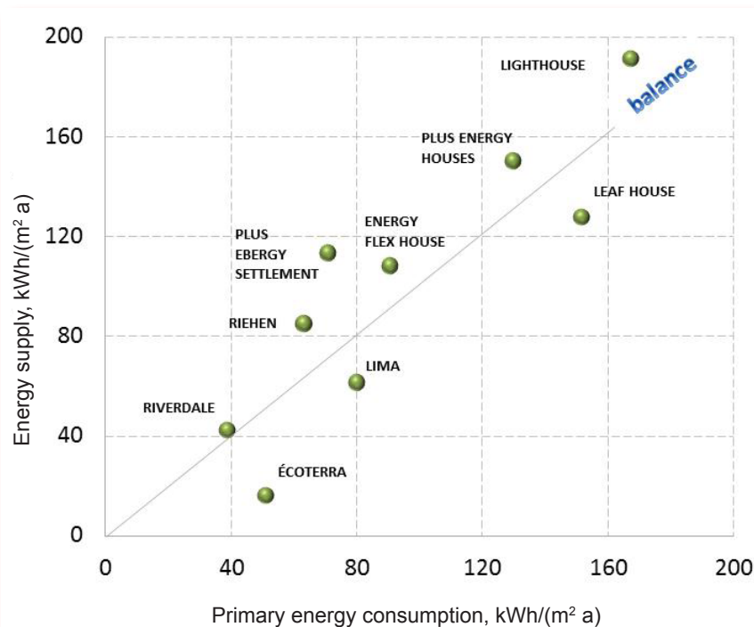
Figure 1. Primary energy consumption and energy supply for the case studies.
