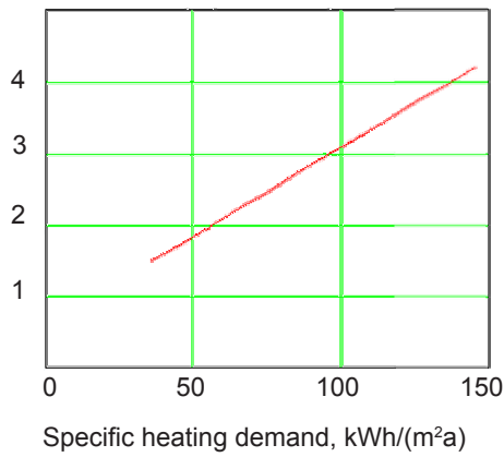
Figure 4. Line density as a function of energy retrofit standard (left) and the resulting specific costs of heat distribution (€/MWh, right). Line density is defined as the amount of thermal energy transported through the neighbourhood distribution grid in MWh/(m a).
