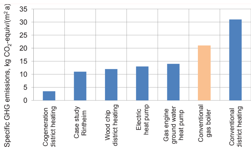
Figure 3. Comparison of optimized building retrofit measures combined with centralised or individual energy supply systems, in terms of GHG emissions (kg CO 2 -equiv/(m 2 a)).
