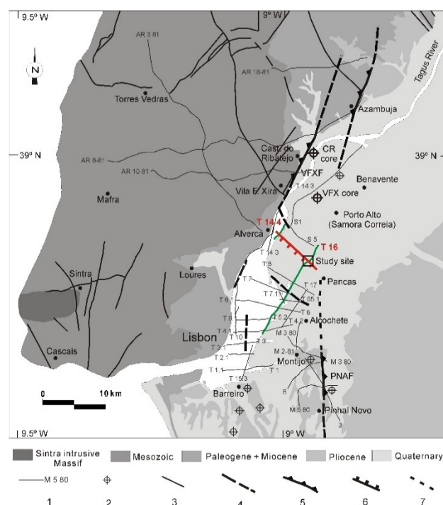
Figure 2. Simplified geological map of the LTV region, showing faults recognised on oil exploration seismic profiles (after Cabral et al. , 2003) and the location of the study site and the Porto Alto fault zone (in red). 1, seismic profile location; 2, oil exploration borehole; 3, previously mapped fault (I.G.M., 1992); 4, fault recognised on seismic section (certain and probable); 5, reverse fault; 6, normal fault; 7, presumed fault trace; PNAF, Pinhal Novo – Alcochete fault; VFXF, Vila Franca de Xira fault; CR core, Castanheira do Ribatejo core; VFX core, Vila Franca de Xira core; in green, seismic lines referred to in the text.
