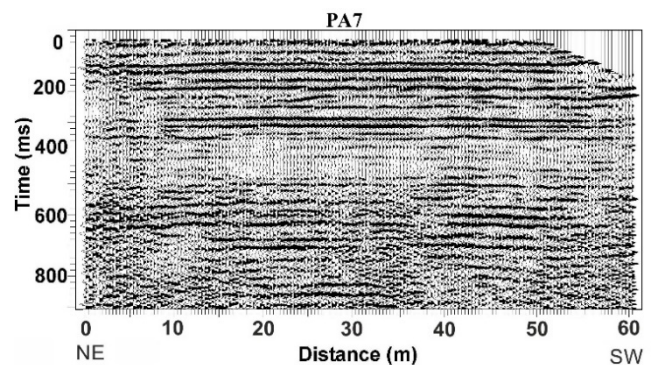
Figure 6. Post-stack migrated shear-wave seismic reflection profile PA7.
