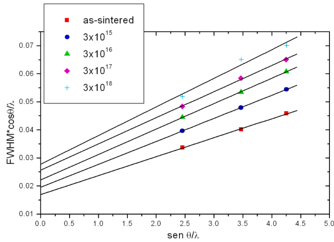
Fig. 6. Representation of \frac{FWHM \cdot \cos(\theta)}{\lambda} as function of the scattering vector norm, \frac{\sin(\theta)}{\lambda} for the three sets of planes (110), (200) and (211). The solid lines represent the linear fit.
