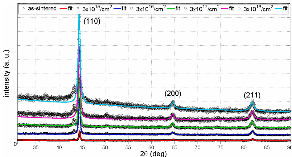
Fig. 5. XRD diffractograms of as-sintered and irradiated samples with the \text{Ar}^+ fluences of 3 \times 10^{15} \text{Ar}^+/\text{cm}^2 , 3 \times 10^{16} \text{Ar}^+/\text{cm}^2 , 3 \times 10^{17} \text{Ar}^+/\text{cm}^2 and 3 \times 10^{18} \text{Ar}^+/\text{cm}^2 . The diffractograms are vertically translated for clarity. Peaks indexed to the dominant phase, i. e. (110), (200) and (211) were fitted using a Marquardt-Levenberg algorithm. Sets of Pseudo-Voigt functions were found to best fit the peaks.
