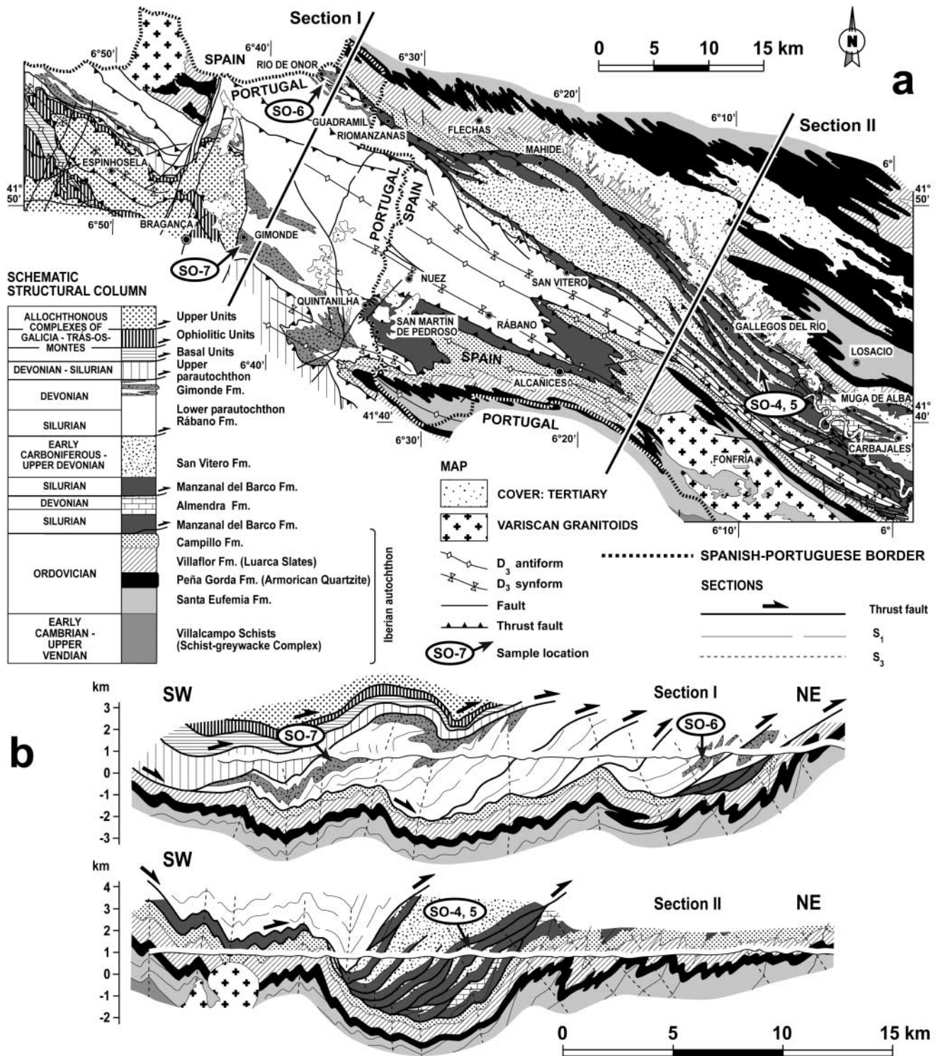
Fig. 3. (a) Geological map of the Alcañices synform showing the sampling localities. The structural column is simplified and shows the main units of the allochthonous and parautochthonous ensembles; however, many more imbricates exist, as shown in the cross-sections. (b) Geological sections. Thin, long lines represent axial surfaces of D 1 recumbent folds and associated cleavage S 1 ; short dashed lines depict the attitude of S 3 crenulation cleavage and D 3 folds. It should be noted that D 1 folds are cut by thrusts (D 2 ) and both are overprinted by later upright folds (D 3 ). Sampling localities have been projected into the closest section to show their structural position.
