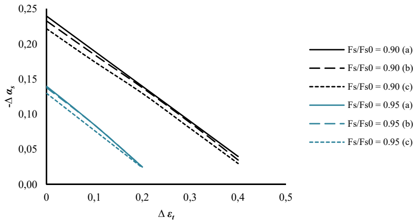
Fig. 2: \Delta\alpha_s versus \Delta\varepsilon_t for the three systems (a, b and c) considered for a system located in Lisbon (latitude = 37.8°)
