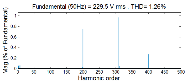
Fig. 21 Voltage distortion with total injected harmonic spectrum, at bus 5, phase 1 for Case IV (T).
