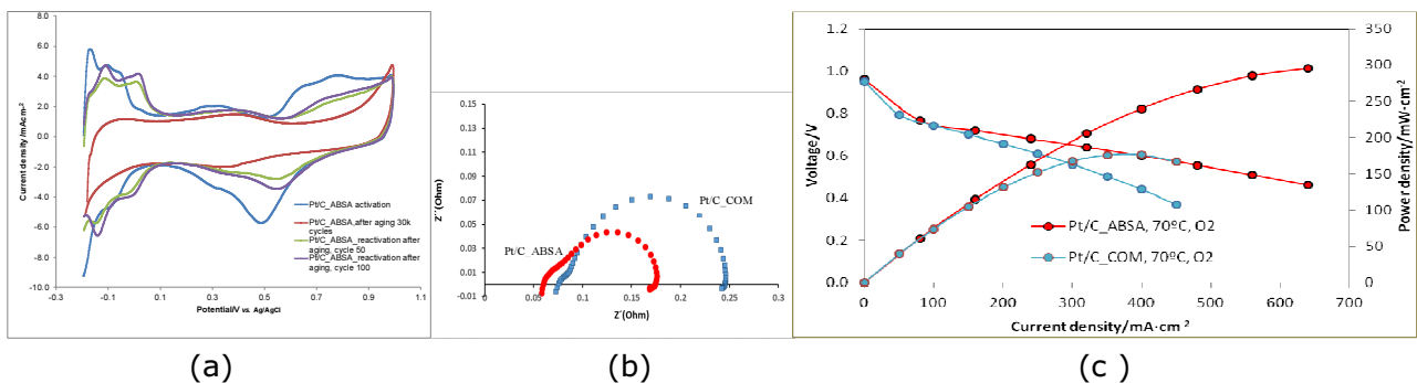
Fig. 1 Half cell : Pt/C_ABSA voltammograms run in 0.5 M H 2 SO 4 at 50 mVs -1 , used to estimate catalyst ESCA after activation, 30000 cycles aging and recovery (a); Full cell : Pt/C_ABSA and Pt/C_COM catalyst, 70°C, oxygen cathode feeding: EIS impedance (b); Polarization and power density curves (c).
