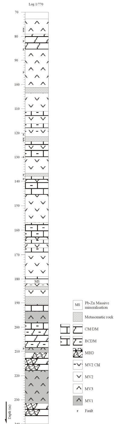
Figura 1 – Metacarbonate-metavolcanic sequence intersected by drill hole SDM-3. Symbols of different rock types as in text.
